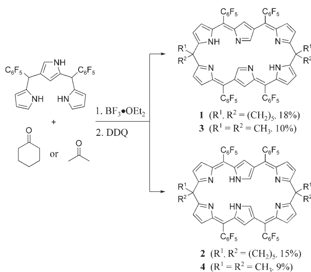
Scheme 1. Synthesis of doubly N-confused calix[6]phyrins(1.1.1.1.1.1).
