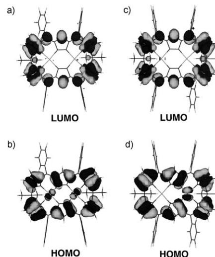
Figure 4. Kohn–Sham orbitals of a) LUMO and b) HOMO of 3-Pt-Pt , and c) LUMO and d) HOMO of 4-Pt-Pt .
