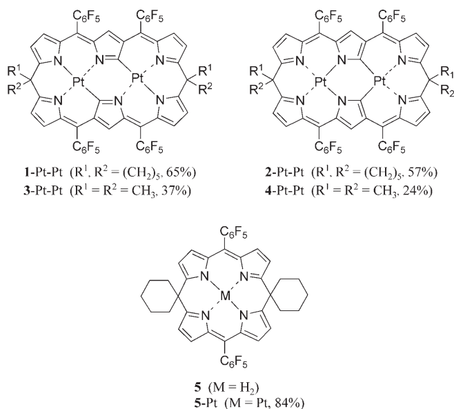
Figure 1. Bis- \text{Pt}^{\text{II}} complexes of doubly N-confused calix[6]pyrins ( 1–4 ) and \text{Pt}^{\text{II}} complex for calix[4]pyrin ( 5 ).
